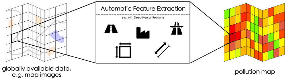
Fig. 1. MapLUR: Automatic feature extraction and globally available data for air pollution modeling. We propose the DOG paradigm (Data-driven, Open, Global) for land-use regression, which advocates openly and globally available data, and automatically extracting features to estimate pollution. Following this newly introduced paradigm, we propose the MapLUR model. It consists of a deep neural network architecture that estimates pollution concentrations for specific locations directly from globally available map images (rendered maps or satellite images), resulting in area spanning pollution maps. For this, MapLUR automatically learns to extract features from the given map images. The extracted features closely resemble manually engineered features for land-use regression models.
